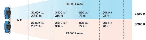
X22 with two S60 Adapters* 1 m / 3.2 ft 3 m / 9.8 ft 6 m / 19.6 ft 10 m / 32.8 ft (High Output)
