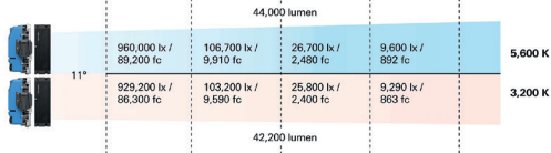
X22 with two X21 Domes 1 m / 3.2 ft 3 m / 9.8 ft 6 m / 19.6 ft 10 m / 32.8 ft (High Output)
